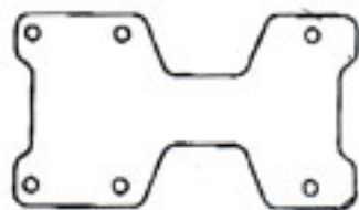
BRAKE PEDAL PLATE
